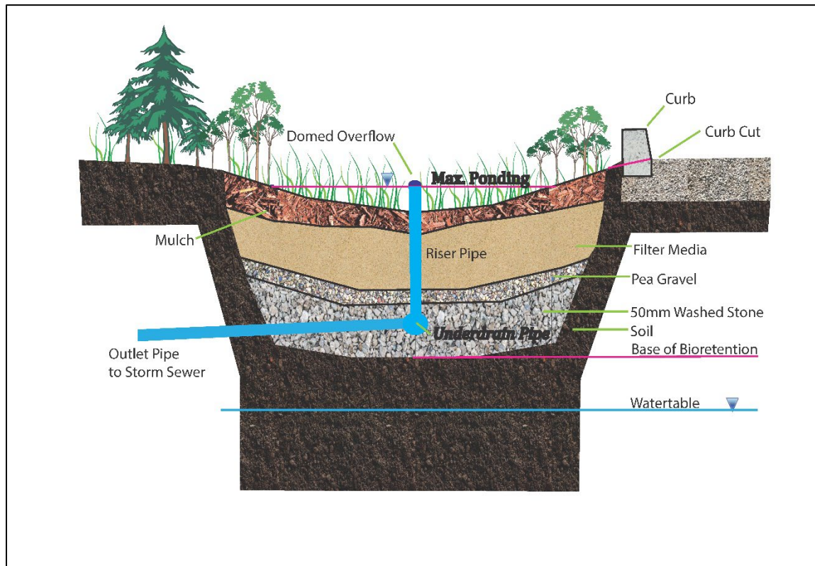
Figure 6-8 - Bioretention
