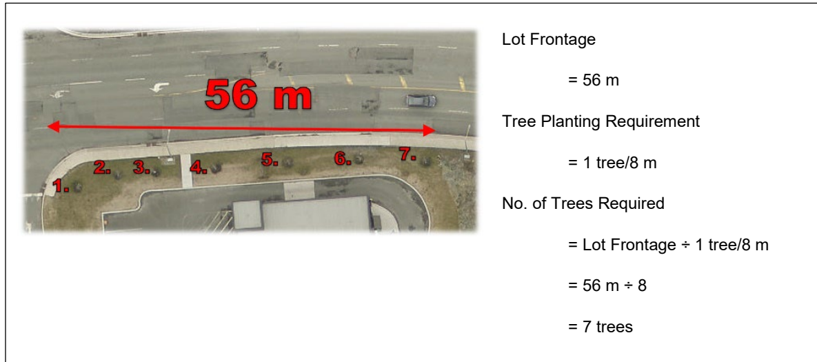
Figure 9-2 - Commercial Tree Planting Example
