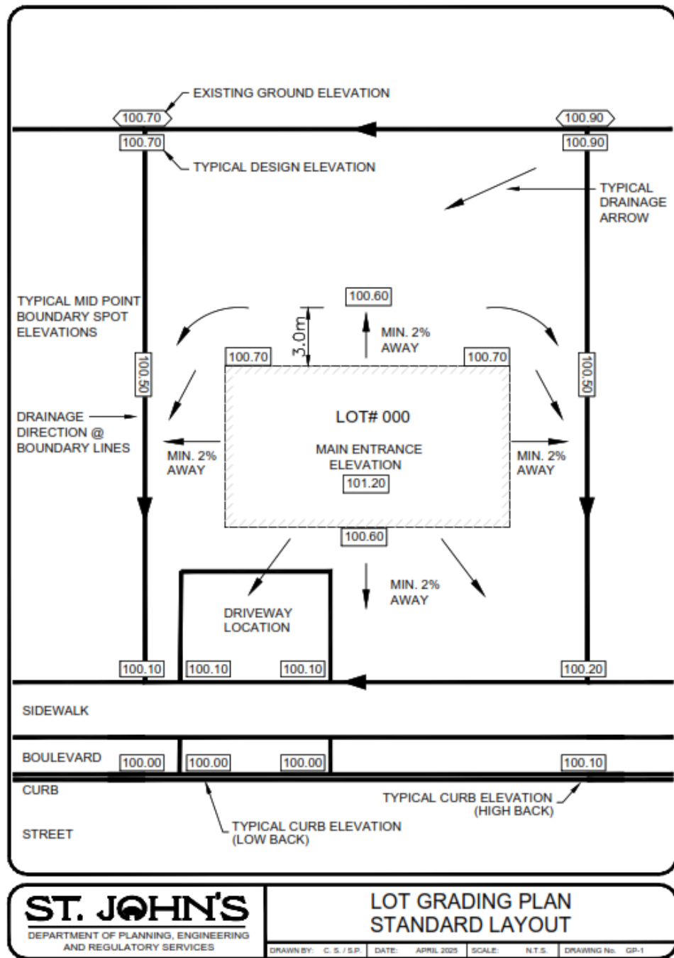
Figure 4-1 - Lot Grading Plan Standard Layout
