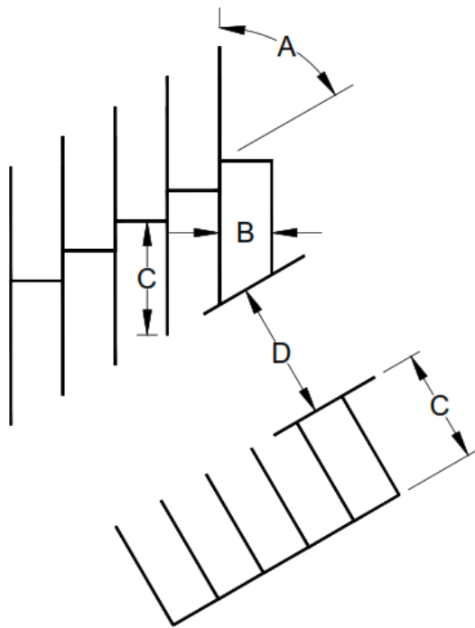
Figure 5-10 - Parking Lot Geometry
