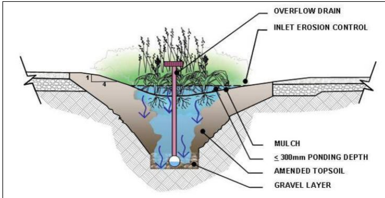
Figure 6-9 - Bioswale
