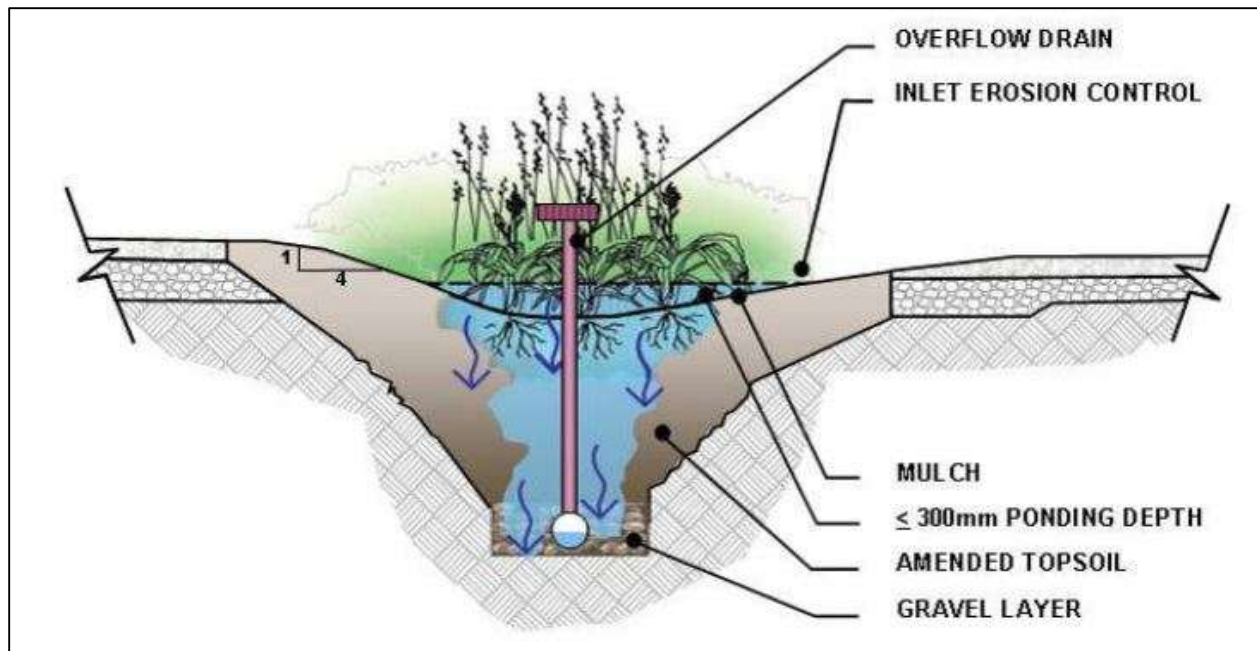
Figure 6-9 - Bioswale
