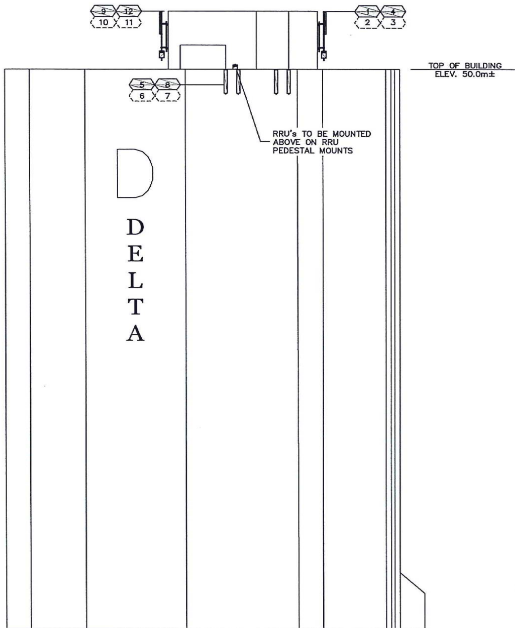
BUILDING LEFT ELEVATION 1:250
